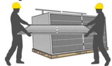
3) Place the metal supporter that is higher or wider than the module in order to avoid hitting and damaging the glass.
